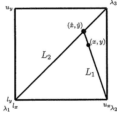
Fig. 4. Depiction of Entities in Proof of Theorem 3
