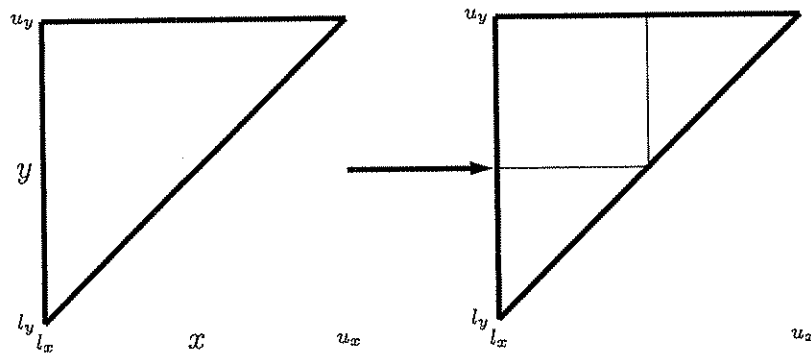
(c) Two-Triangle-Rectangle Partition
