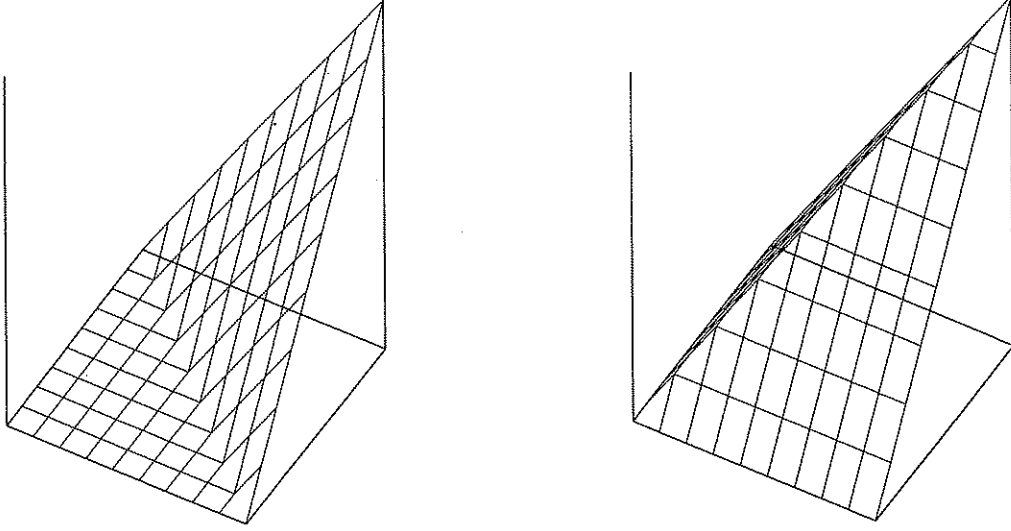
Fig. 2. Convex and Concave Envelopes of xy Over a Rectangle
