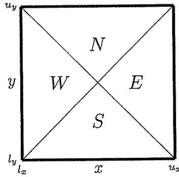
Fig. 3. Pictorial Description of Triangular Regions Studied
