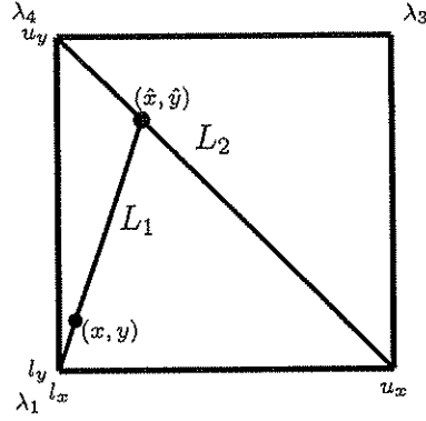
Fig. 6. Depiction of Entities in Proof of Theorem ??
