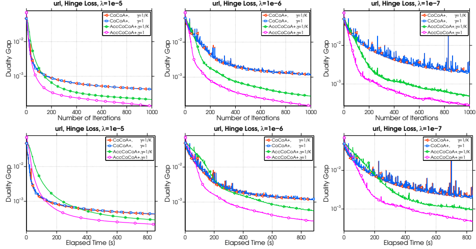
Figure 2: Duality gap as a function of iterations (top row) and elapsed time (bottom row) when solving hinge-loss SVM problems with different regularization values ( \lambda ) on the url dataset.
