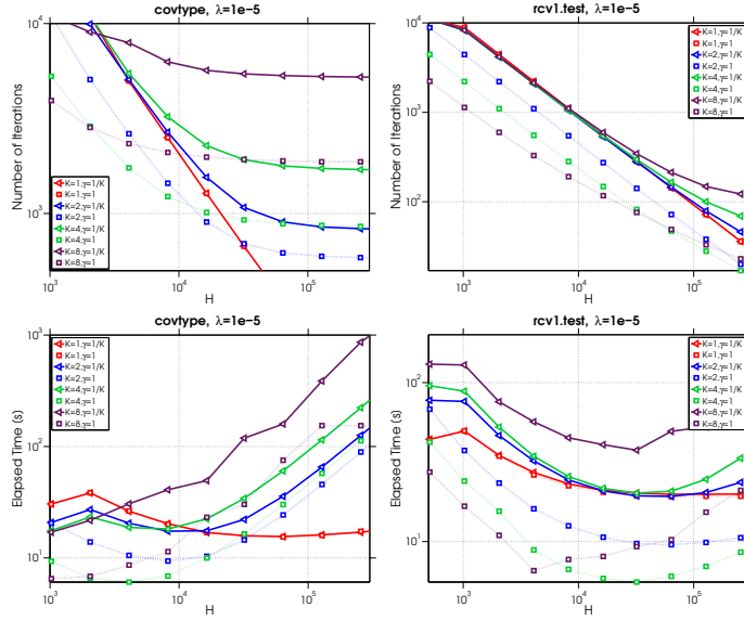
Figure 5: Number of iterations and running time required to reach a tolerance of 10^{-3} on the duality gap as the inner iteration limit ( H ) is varied.
