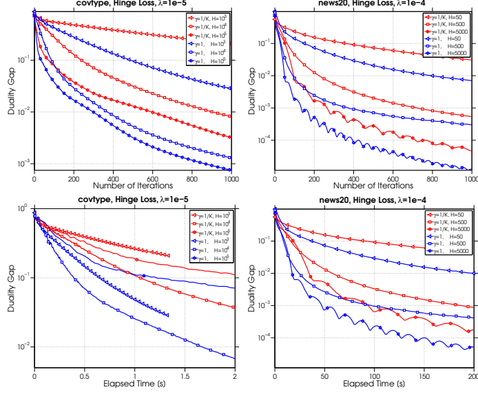
Figure 4: Comparison of performance for different inner iteration limits when \sigma' = \frac{1}{K} and \sigma' = 1 .
