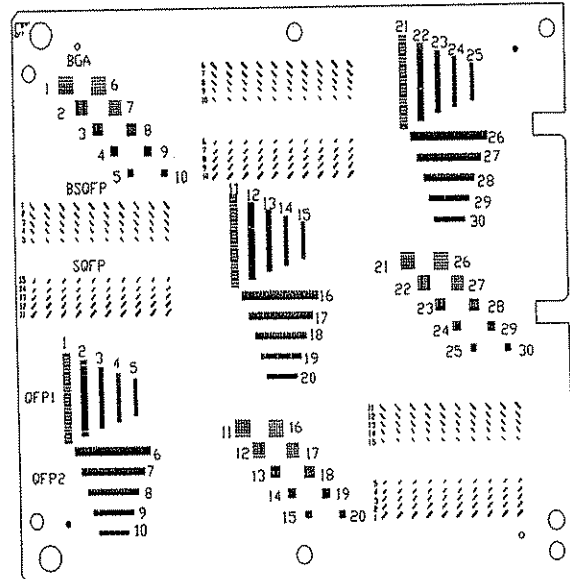
Figure 2. Test Pattern of Stencils and FR-4 Boards
