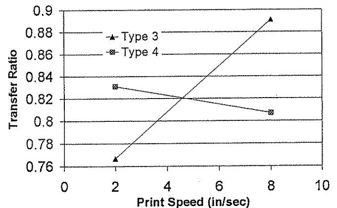
Figure 9. Interaction plot of solder type and print speed for QFP apertures
