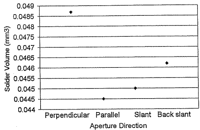
Figure 8. Solder Volume vs. Aperture Shape
