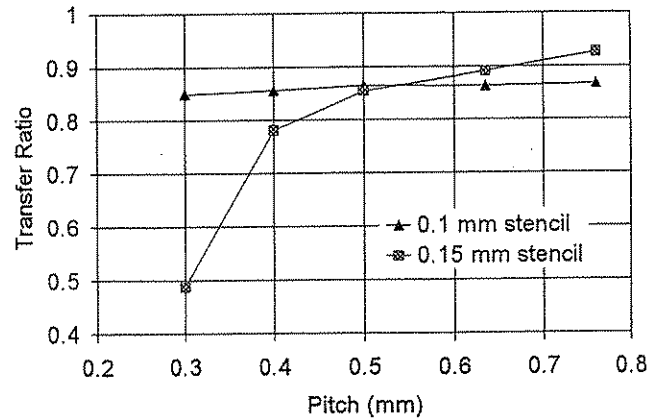
Figure 5. Transfer ratio vs. Pitch for QFP apertures
