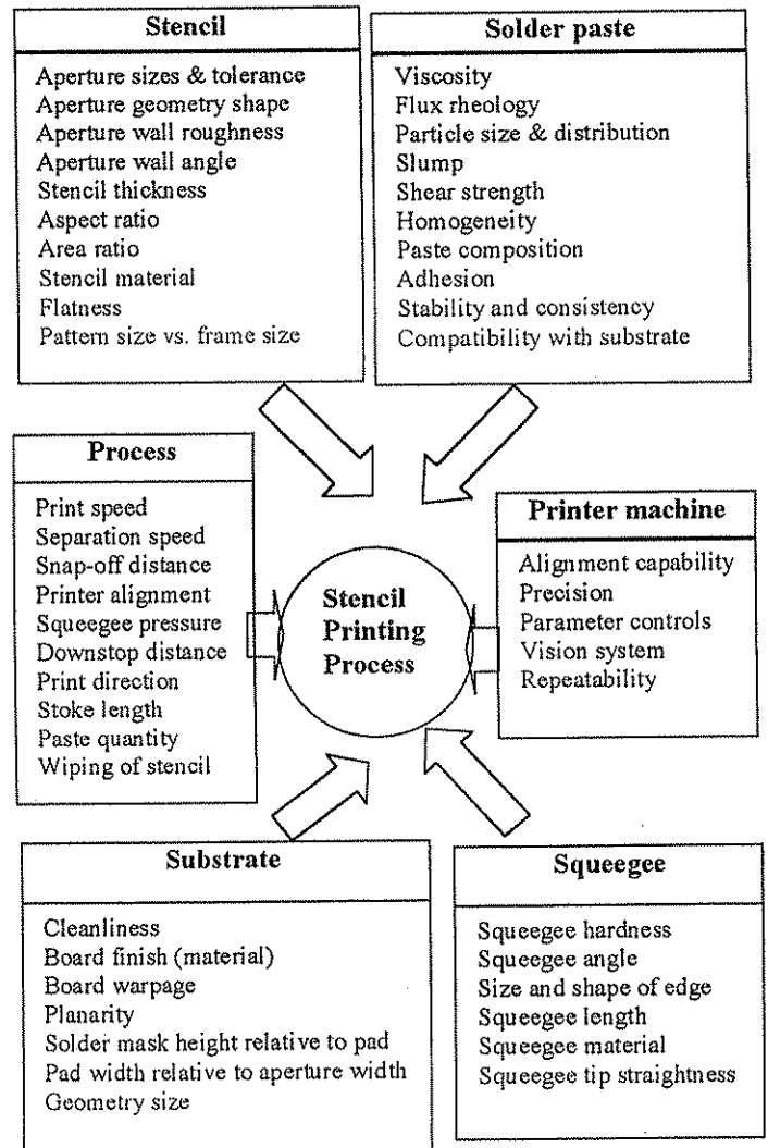
Figure 1. Factors that influence the stencil printing process
