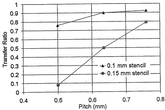
Figure 6. Transfer Ratio vs. Pitch for BGA Apertures
