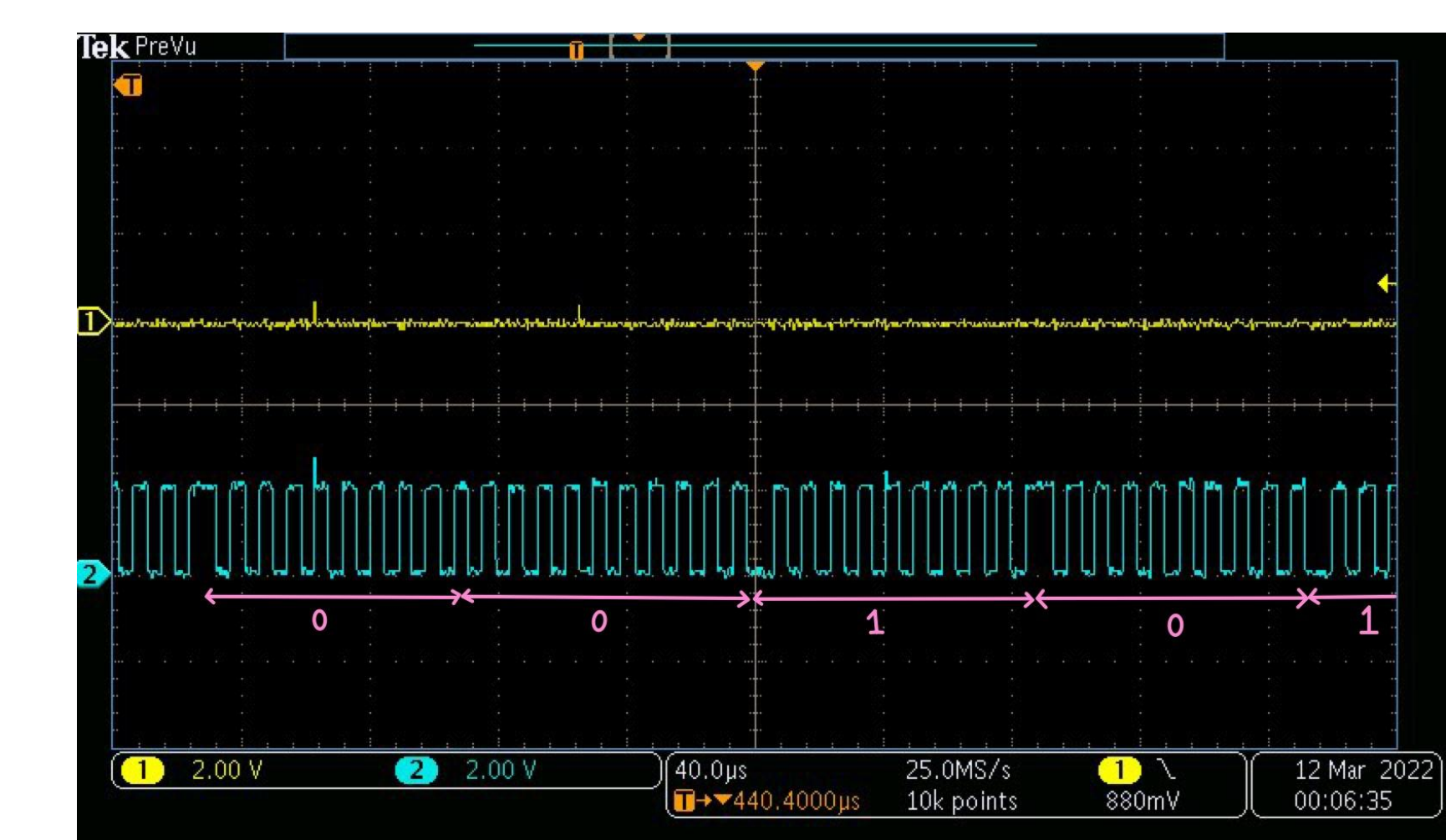
Figure 8: Break down of the bit by bit modulation for each symbol in 10 cycles. Shows how one bit is read by 10 cycles of a repeating phase state.
