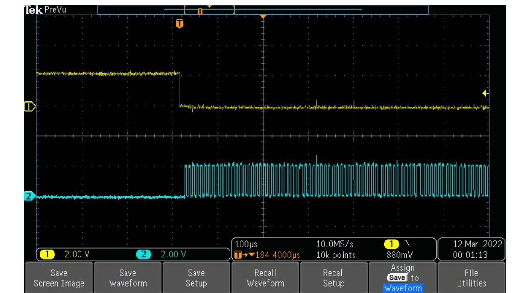
Figure 7: Snapshot of output of modulated signal. The yellow line shows when the modulation cycle is free or not, so when low, it is in use and not free. Here the modulation can be seen in the output wave depicted by the blue square wave.
