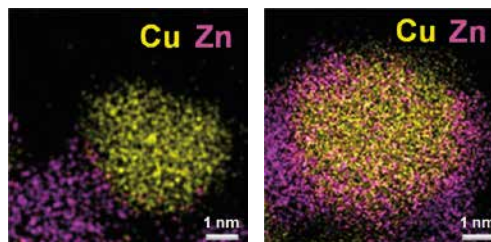
At left, the catalysts are mostly present as separate particles after activation with molecular hydrogen. At right, zinc oxide “decorates” metallic copper particles after induced activation.
